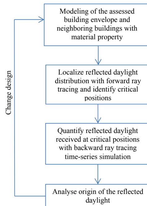
Figure 1 Flowchart of the reflected daylight evaluation procedure.
