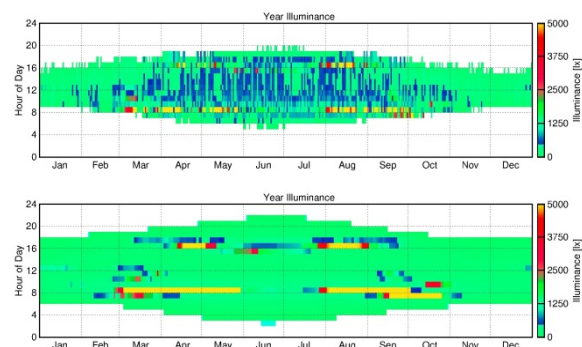
Figure 6 Heat map of illuminance received at one critical position with different weather condition. Top: weather data for Geneva. Bottom: CIE clear sky.
